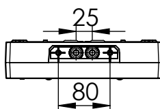
Wandmontage
